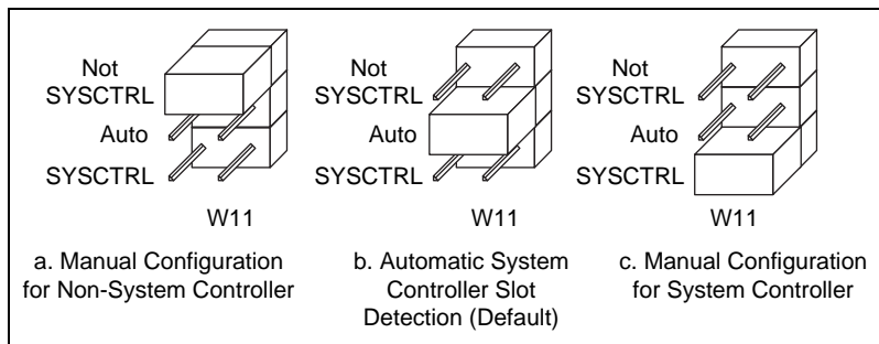
Figure 3-4. System Controller Slot Configuration
